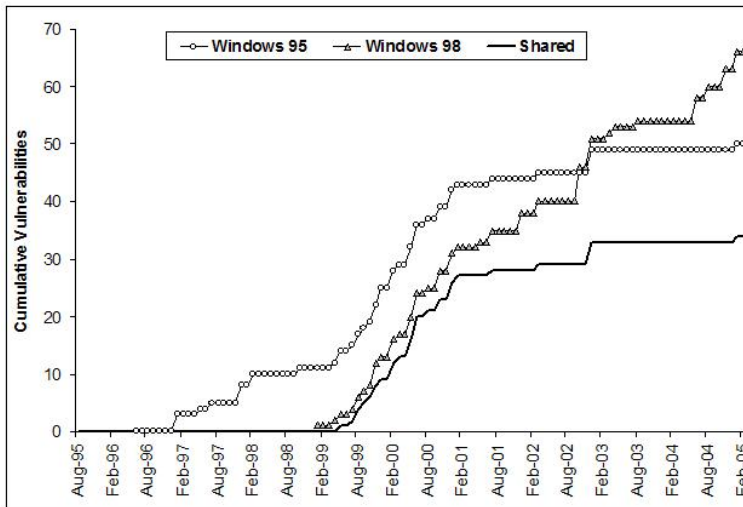
Fig. 1. Cumulative vulnerabilities in Windows 95 and Windows 98
