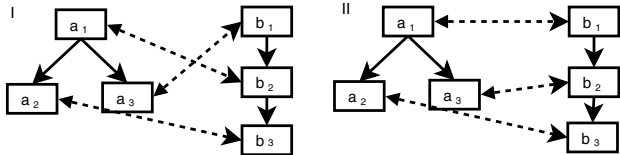
Fig. 4. I.A mapping with semantic contradiction; II. A harmonic mapping
